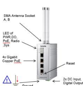
JetWave 2714G-WIFI
