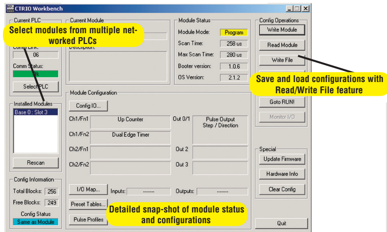
CTRIO Workbench main configuration screen
